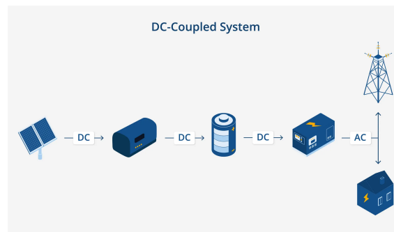
Figure 1.2: DC-coupled battery energy storage system diagram. Source: RatedPower
