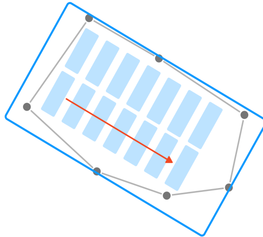
Figure 2.3: Optimized rotation angle of the BESS layout. Source: RatedPower
