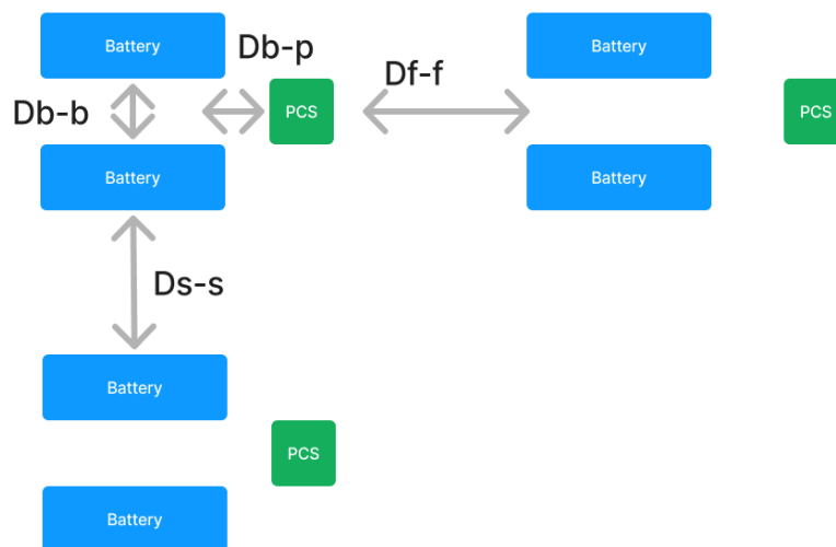
Figure 2.2: Safety distances between battery power blocks. Source: RatedPower
