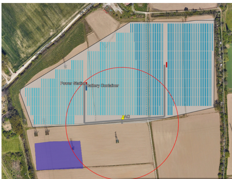
Figure 3.2: The battery containers are connected to the power station closest to the MV point. Source: RatedPower
