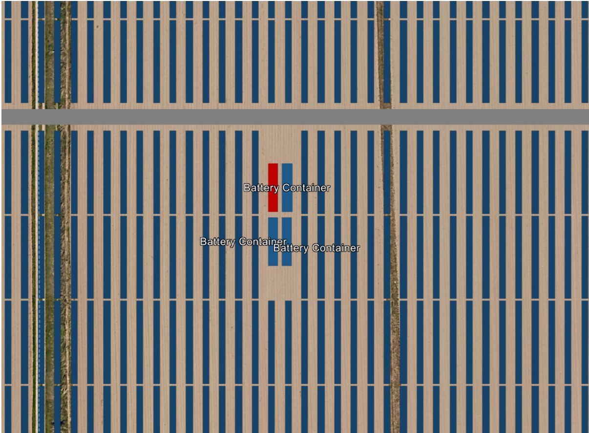
Figure 3.5: Power station and battery container located inside the DC solar field. Source: Rated-Power
