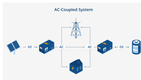
Figure 1.1: AC-coupled battery energy storage system diagram. Source: RatedPower
